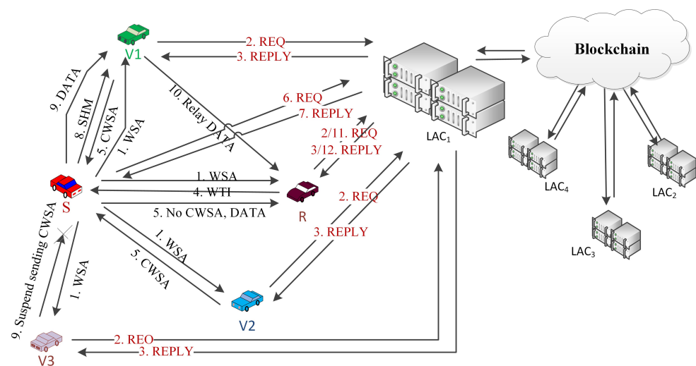
Figure 5. A sample scenario presenting GMT.
