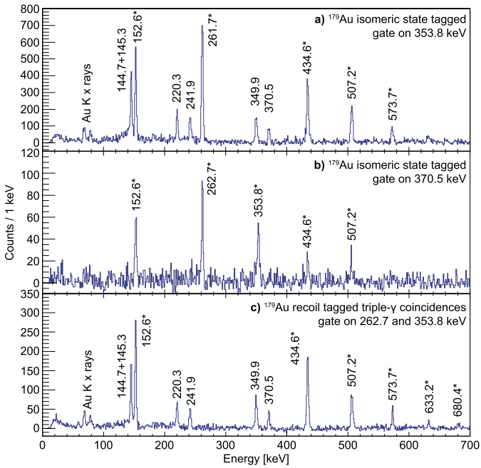
Fig. 2. Spectra of \gamma rays of ^{179}\text{Au} a) tagged with decay of the 326 ns isomer and in prompt coincidence with the 353.8 keV transition, b) tagged with decay of the 326 ns isomer and in prompt coincidence with the 370.5 keV transition, and c) in prompt coincidence with the both 353.8 and 262.7 keV (without tagging). Transitions of the yrast 1i_{13/2} band are denoted with an asterisk.
