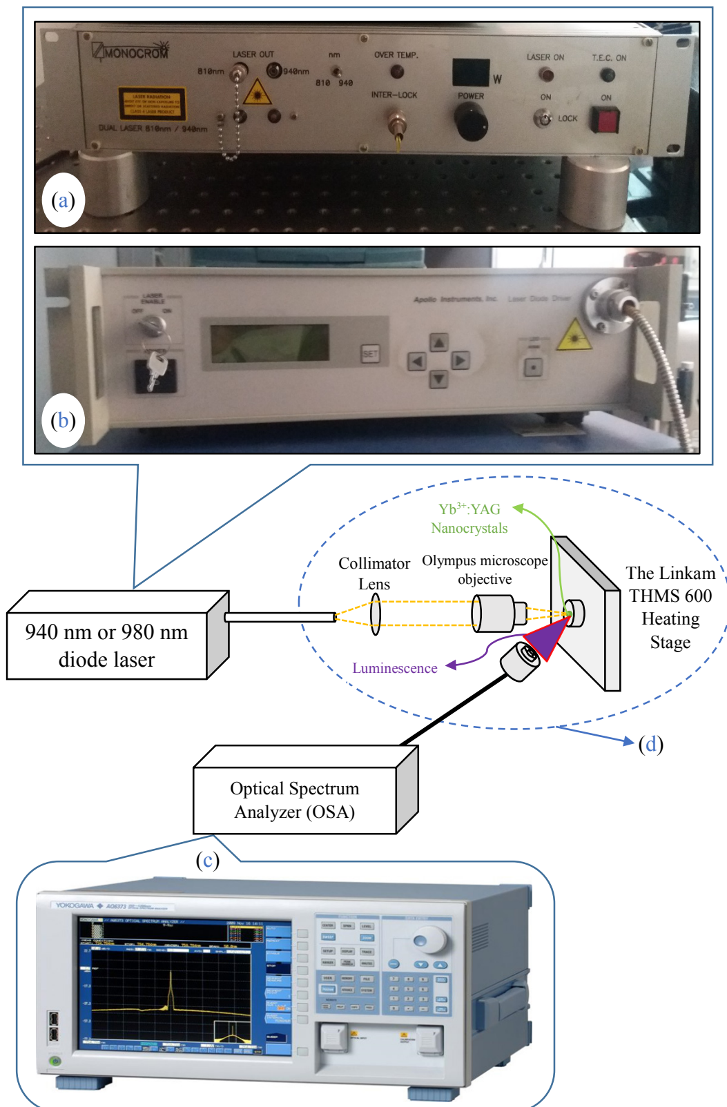
Figure 2.14. Scheme of fluorescence intensity ratio (FIR) setup. (a) picture of the fiber-coupled MONOCROM dual-wavelength diode laser, 808nm / 940nm, (b) Picture of 980 nm InGaAs diode laser (Apollo Instrument, Inc. S50-980-2) connected to an optical fiber with a 20 \mu\text{m} core diameter as the excitation light source, (c) Picture of a Yokogawa AQ6373 Series optical spectrum analyser (OSA), (d) Scheme of the the Linkam THMS 600 heating stage, Olympus microscope objective, Collimation lens, and the other optical components.
